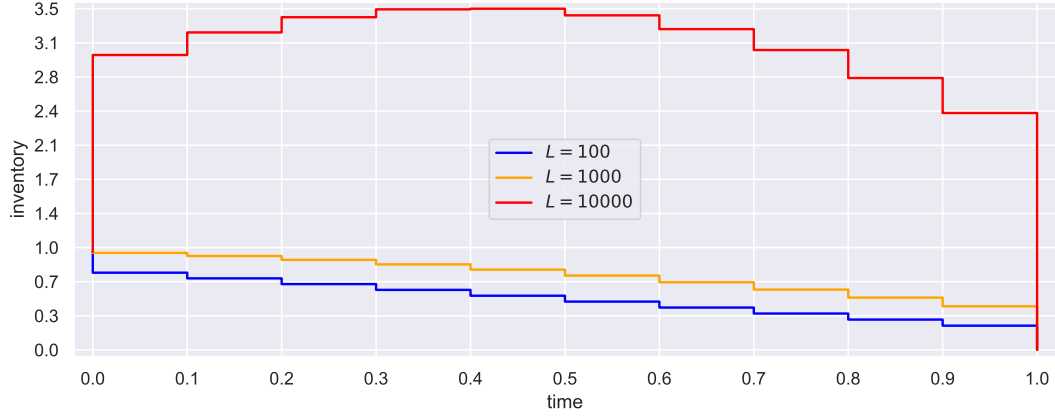
(a) Influence of L ; \mu = 0.001
