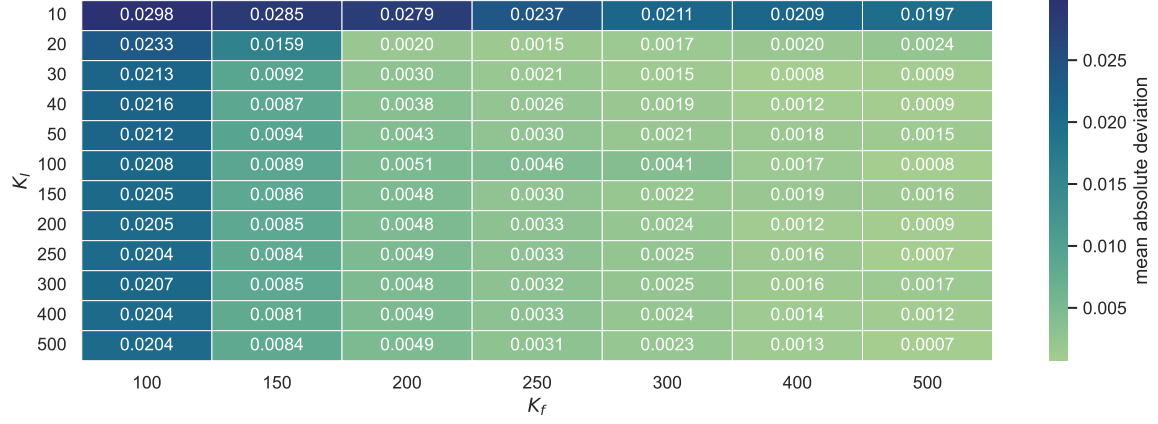
(a) Mean absolute error
