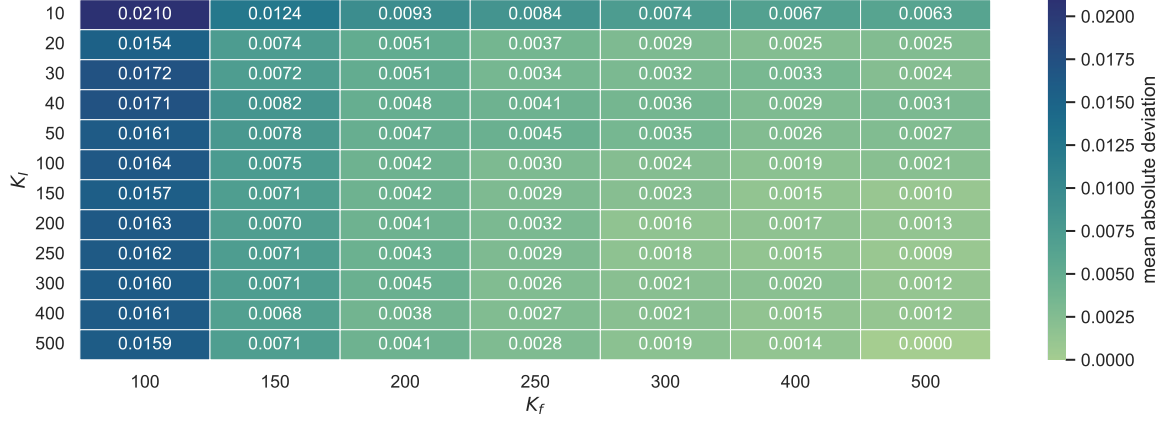
(a) Mean absolute deviation
