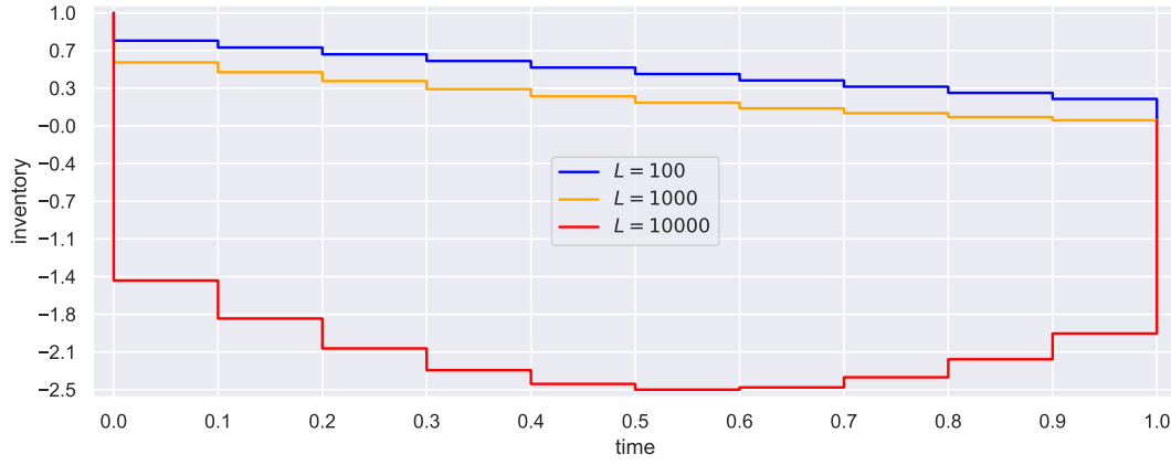
(b) Influence of L ; \mu = -0.001
